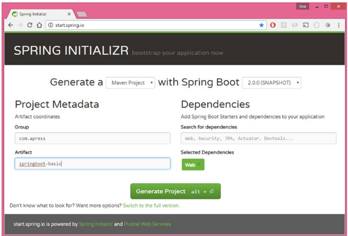
Figure 2-1. Spring Initializr
